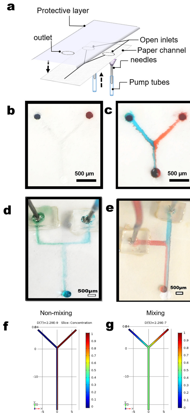
FIG. 3. Paper-based open-channel microfluidic devices derived from TACH. (a) Schematic assembly of a device. A fabricated device before (b) and after (c) introducing liquid in the channel at 0.1 ml/min flow rate. (d) and (e) Top inlet designs of TACH performed showing laminar flow on different designs and dimensions. (f) and (g) Concentration evolution along the length of a cross-section of the channel from the inlet (top) to the outlet (bottom). Almost non-mixing (left for Pe = 8.6 \times 10^6 ) or mixing (right for Pe = 0.86 ) operating conditions can either be selected, validating the possibility to use paper for microfluidics devices.
